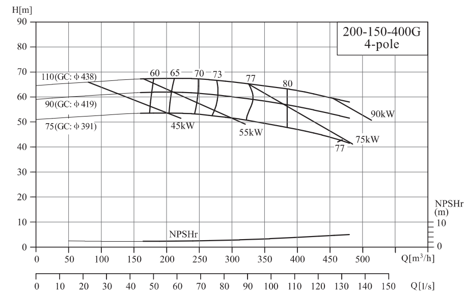
NIS200-150-400G
