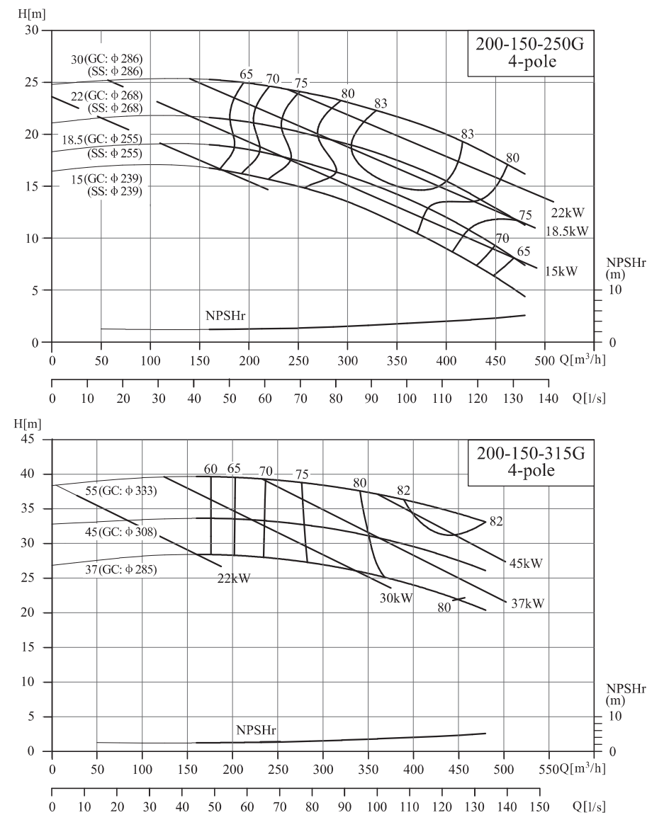
NIS200-150-250G/200-150-315G
