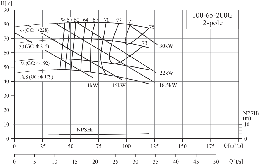
NIS100-65-200G/100-65-250G
