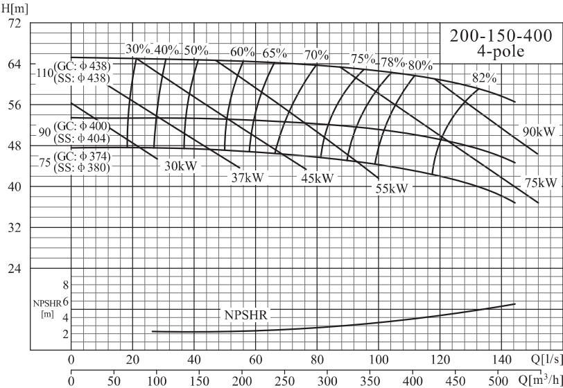
NISO,NIS,NISF 200-150-400/250-200-315
